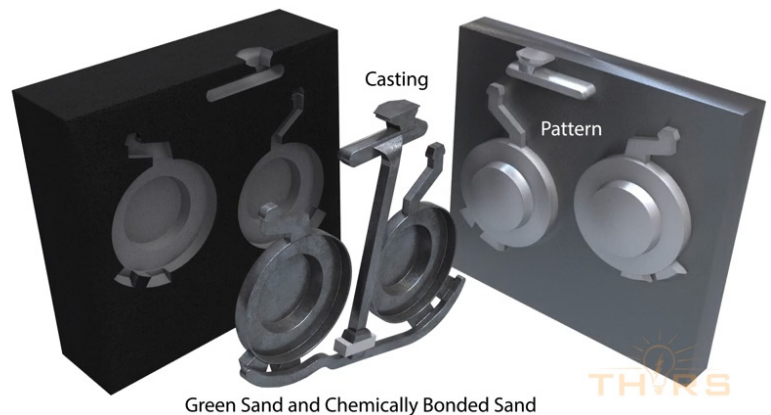
Green Sand and Chemically Bonded Sand
